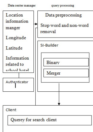
Fig.1. The architecture of keyword search using spatial inverted index
