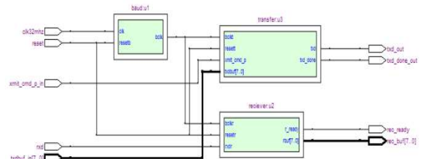
Fig 3.4 -: RTL of Top File
