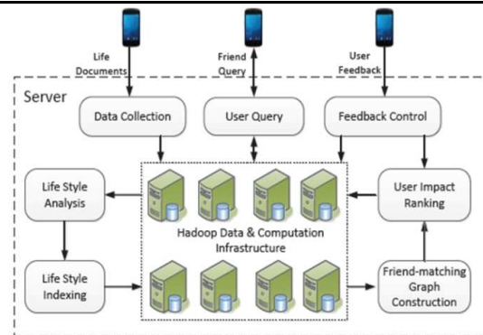
Fig.1. architecture of friend book service
