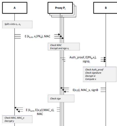
Fig.3. Collaborative two-pass key transport.
