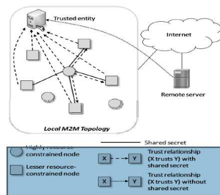
Fig.2. Network model and assumptions.
