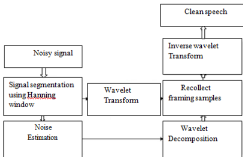
Figure 8: Block diagram of wavelet decomposition
