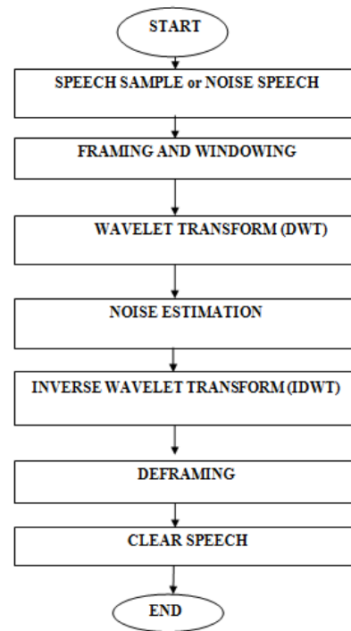
Figure 9: DWT Flow Chart
