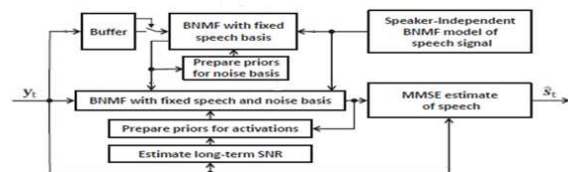
Figure 2: Block diagram representation of BNMF.
