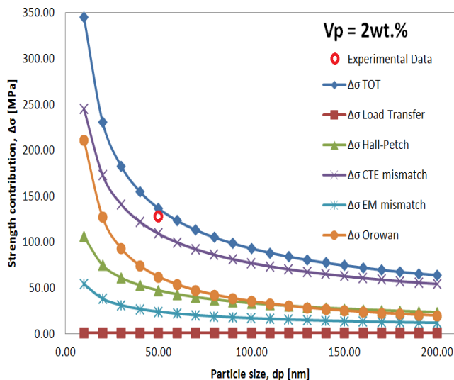
Figure 1. Effect of strengthening contributions and total resulting strengthening increment calculated by Equation (10) for a 2 wt.% Al 2 O 3 reinforced Al matrix composite.
