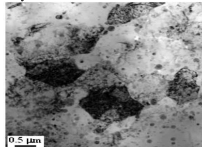
Figure 4. TEM microstructure of the Al-10 wt%Al 2 O 3 nanocomposite showing the homogeneous dispersion of Al 2 O 3 nanoparticles (<50 nm in sizes) in the Al matrix.
