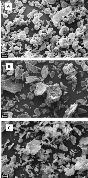
Figure 3. SEM micrographs (secondary electrons) of pure aluminum powder (A) as received, (B) after 2 h of ball milling and (C) after 5 h of ball milling.
