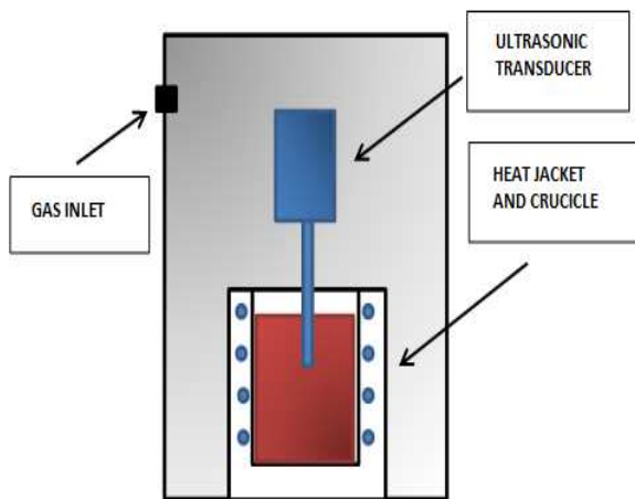
Figure 2. Scheme of experimental setup used by X. Li et al.
