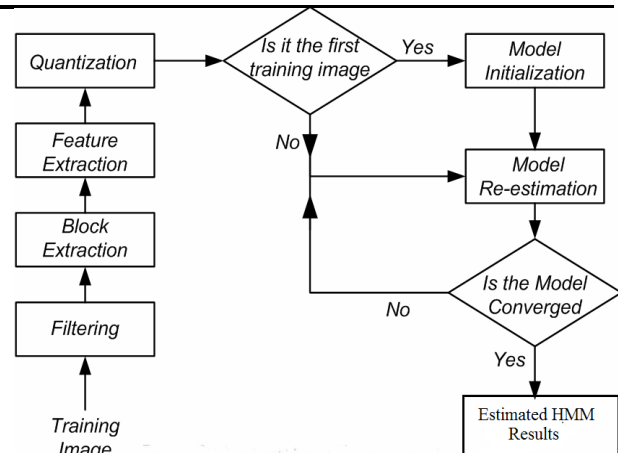
Fig 2. Block diagram of training procedure
