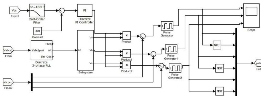
Fig: (B) Controller Simulink diagram
