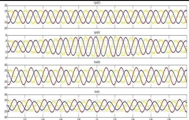
Fig.4: Simulation results: (a) Grid voltages, (b) Grid Currents (c) Unbalanced load currents, (d) Inverter Currents
