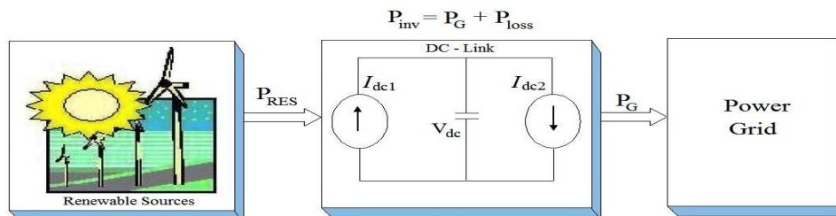
Fig. 2: DC-Link equivalent diagram.
