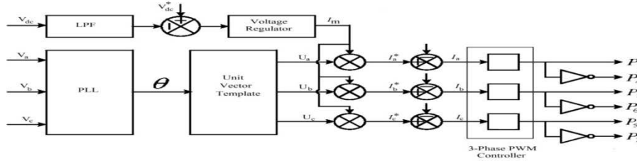
Fig. 3: Block diagram representation of grid-interfacing inverter control.
