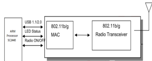
Fig. 4 The interface block diagram of Wi-Fi transmitter
