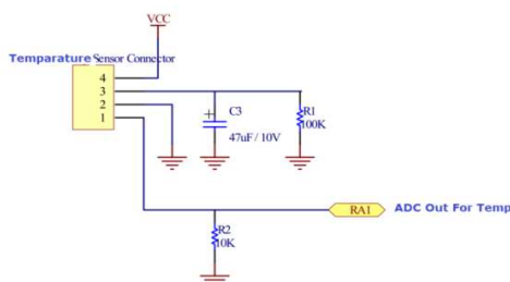
Fig.3 The Interface Block Diagram Of HSM20G
