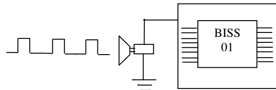
Figure 4. Ultrasonic Sensor with Controller
