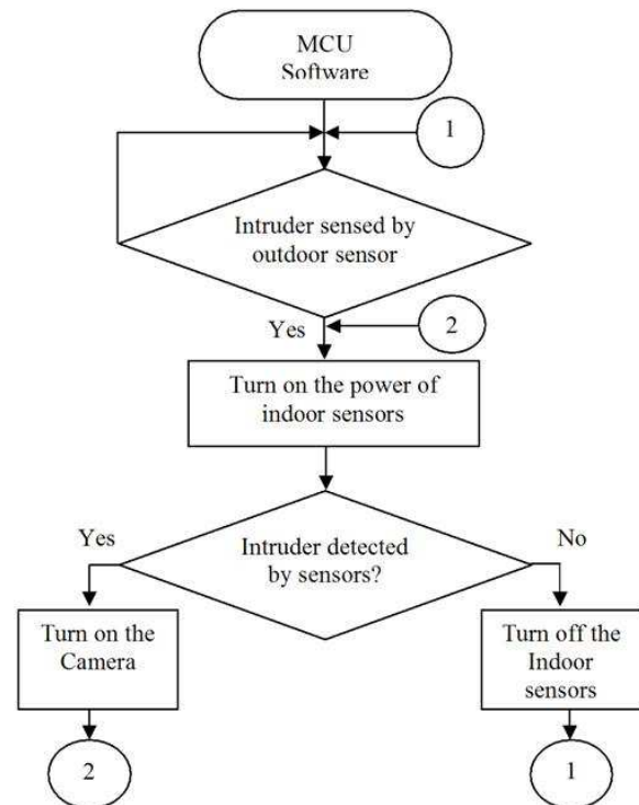
Figure 5. Software flowchart
